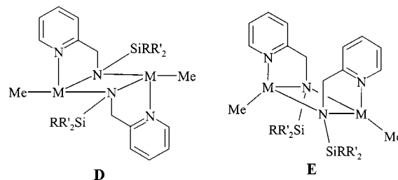
Scheme 6. Schematic drawing of the two possible conformations D and E for the dimeric derivatives of the type [\text{R}-\text{M}-\text{N}(\text{SiRR}'_2)\text{CH}_2\text{-py}]_2 with M as Zn ( 2 and II ) and Mg ( 7 and 9 )
